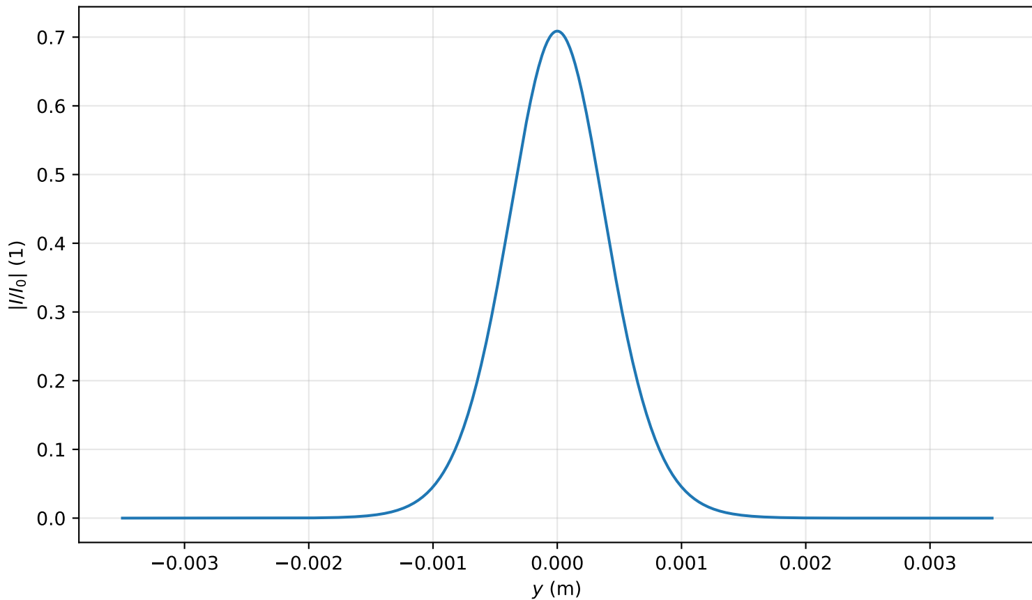
Intensity profile I(x=0, y, z=2.070)/I_0 , P_{in}=0.4P_{cr} , artificial time
